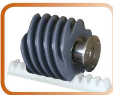
The energy-efficient patented worm drive requires NO grease or lubricants.
